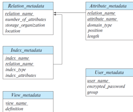
Relational schema representing part of the system metadata.
